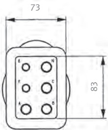
Type 14 Plug
