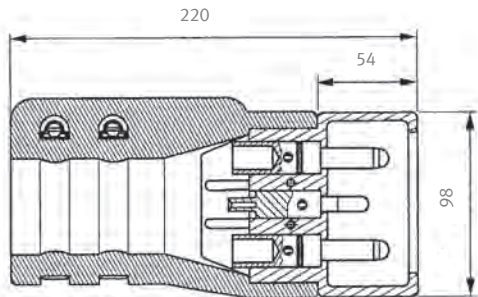
Type 14 Plug
