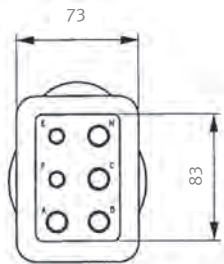
Type 14 Plug
